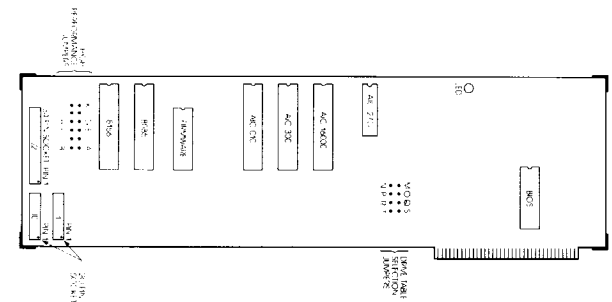
Figure 1. Board Layout
