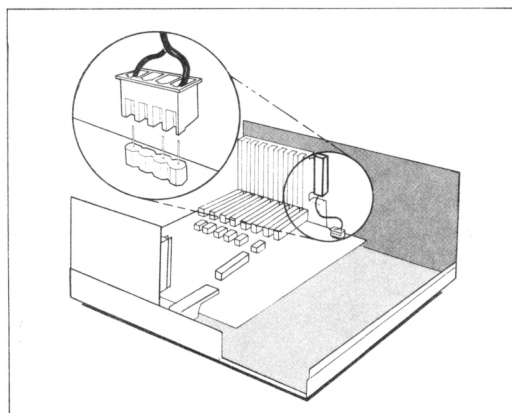
Connecting Battery to System Board
