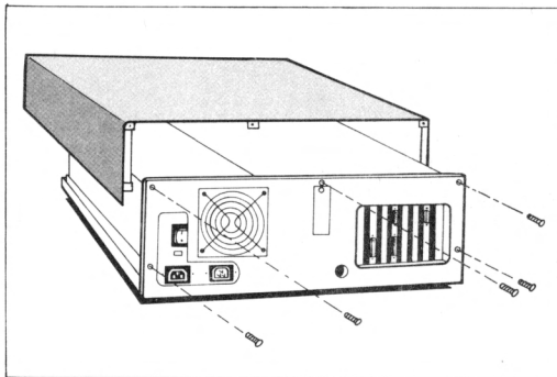
Removing Screws
