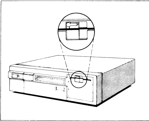
Diskette Drives
