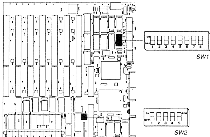
Locations of the DIP Switches
