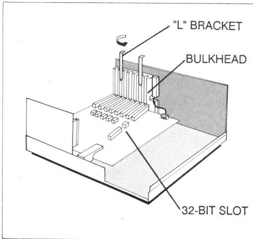
Expansion Slots
