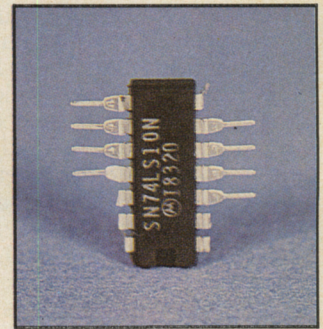
RIGHT: The prepared "piggyback" IC for location ZM9 (74LS10) is shown after its pins have been formed (or removed) per the instructions in the text.
