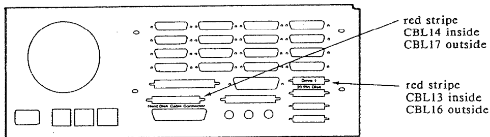
Figure 3. COMPUTER ENCLOSURE - (back panel outside)
