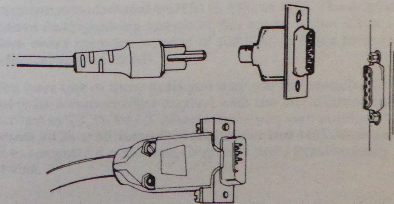
Figure 5.3 Details of Video Connectors and Composite Adapter
