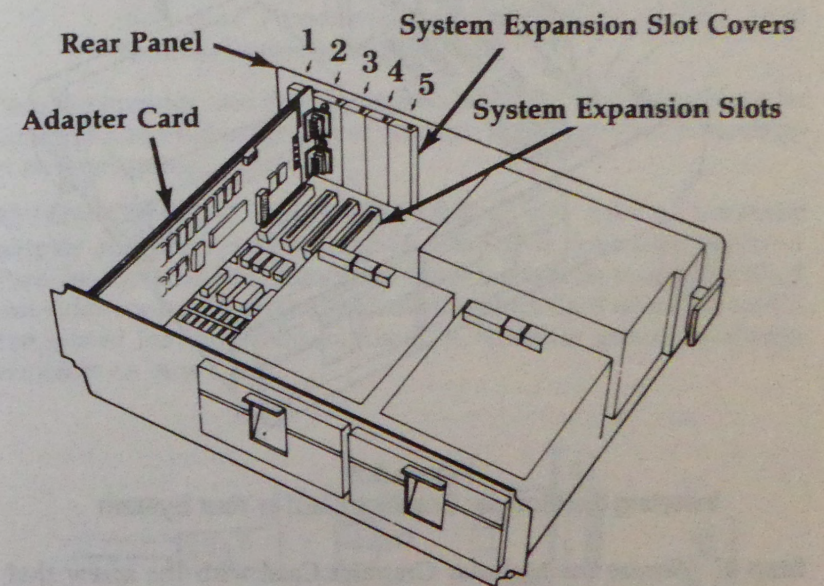
Figure 5.1 Details of Expansion Slots
