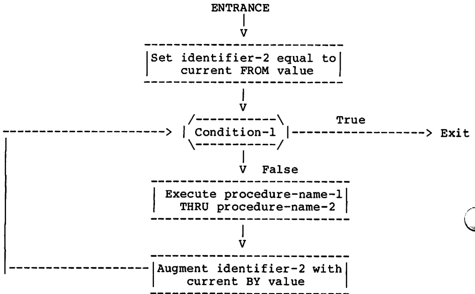
Flowchart for the VARYING Phrase of a PERFORM Statement Having One Condition.
