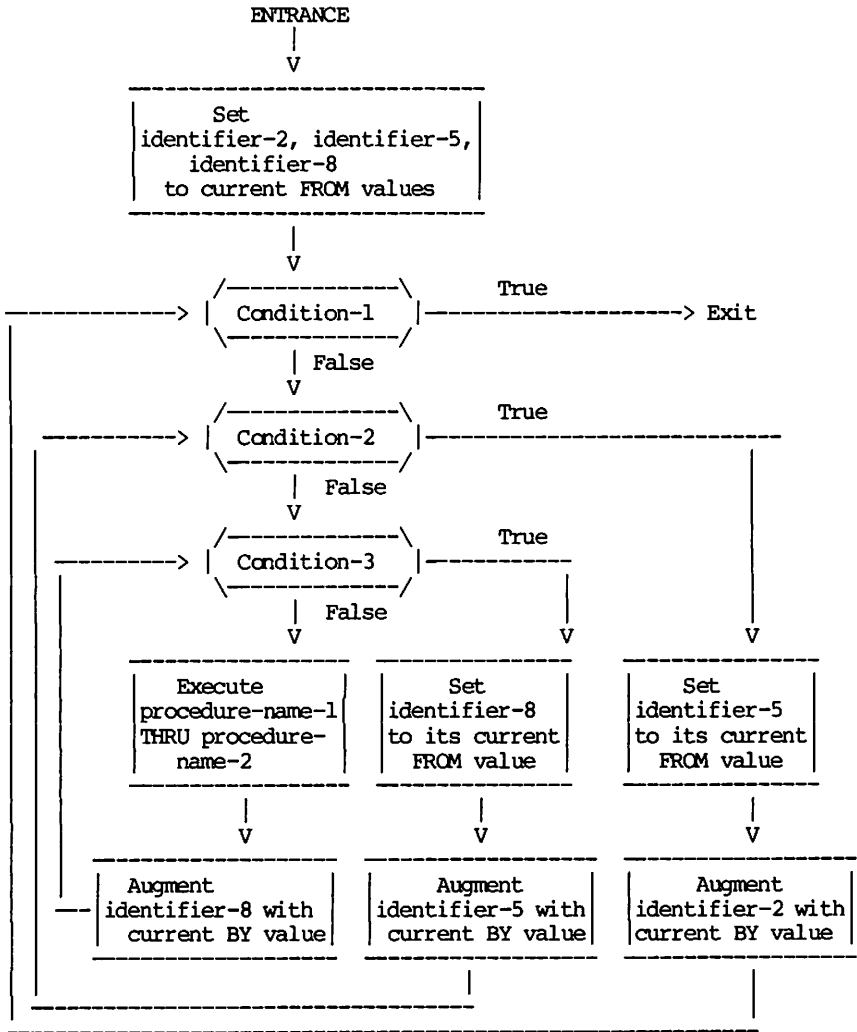
Flowchart for the VARYING Phrase of a PERFORM Statement Having Three Conditions.
