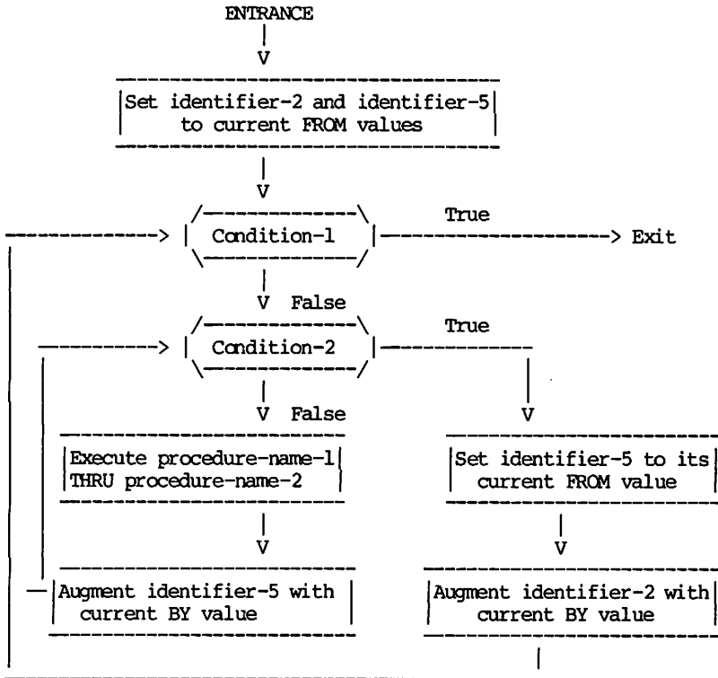
Flowchart for the VARYING Phrase of a PERFORM Statement Having Two conditions.
